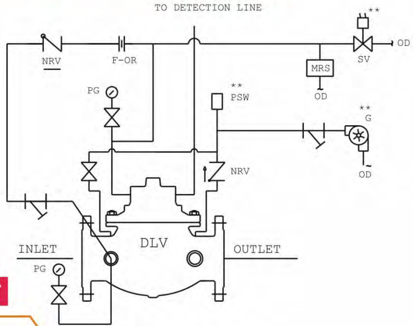
SCHEMATIC-11 FTDLV-WPT-TST
